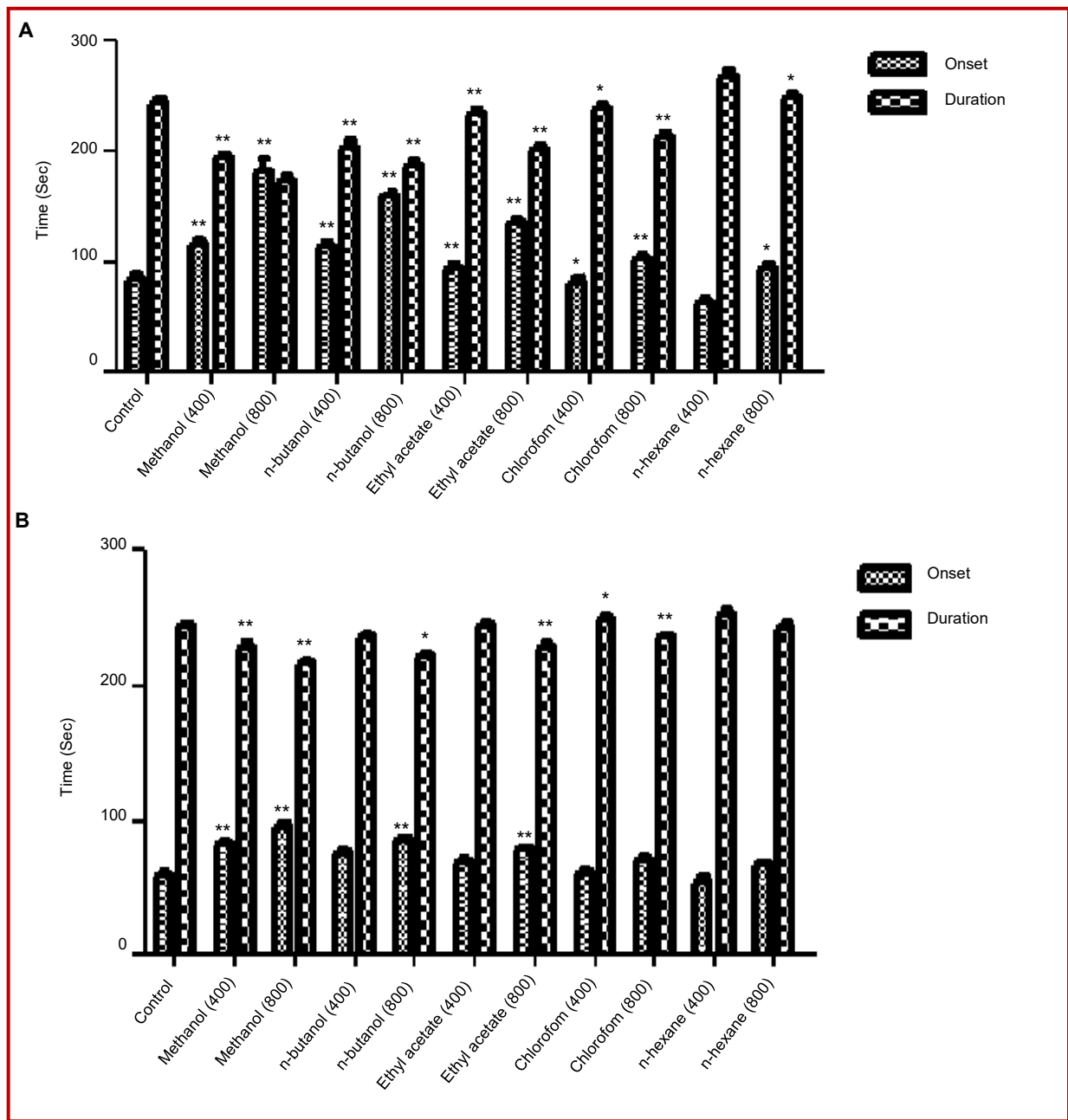
Figure 1: Anticonvulsant effect of A. rosea extract and fractions against PTZ (A)-, strychnine (B)- and picrotoxin (C)-induced convulsions; Mean ± SEM; n=6; *p<0.05, **p<0.01 when compared with control
