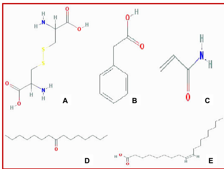
Figure 3: 2D structure of phytocompounds of R. mucronata (A) cystine (B) phenyl acetic acid (C) acrylamide (D) caprylone (E) oleic acid. The structure retrieved from PubChem database
