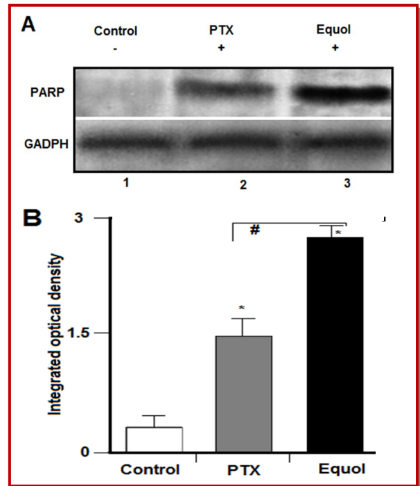
Figure 7: Representative immunoblot and quantitative analysis of PARP protein expression. (A) Western blot analysis showing cleavage of PARP in SKOV-3 cells upon treatment with an IC_{50} dose of equol and PTX. The PARP was detected using specific antibodies. Rabbit Anti-PARP-1 (cleaved p25) monoclonal antibody was attached to the secondary goat anti-rabbit antibody, conjugated with alkaline phosphatase at a dilution of 1/2000. Rabbit anti-GAPDH antibodies were used as internal controls. The blot was developed with BCIP/NBT. (B) The densitometric volume of the PARP bands is expressed relative to the densitometric volume of the loading control gene GAPDH
