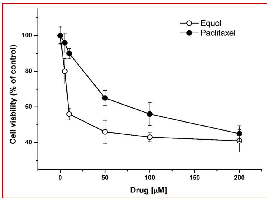
Figure 1: MTT assay results
