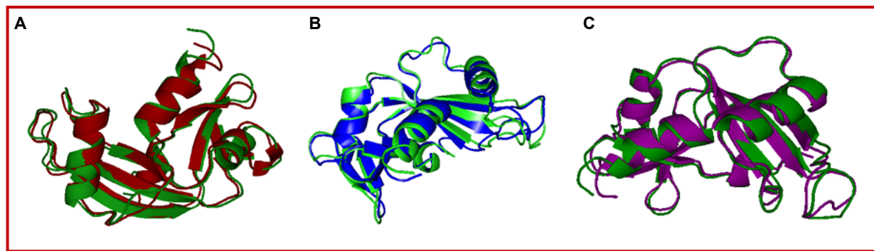
Figure 2: Superimposed structure of the native protein (green) with mutant
