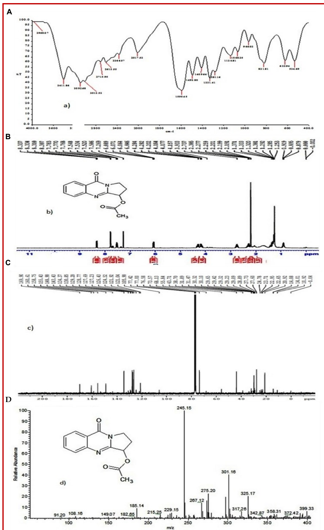
Figure 2: A) FT-IR Spectrum, B) ^1\text{H} NMR, C) ^{13}\text{C} NMR and D) LC-MS of VA-1 compound
